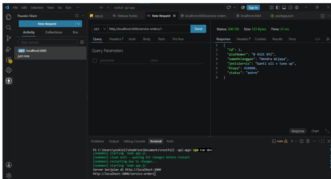
Gambar 3. Pengujian GET //service-orders/1 .
