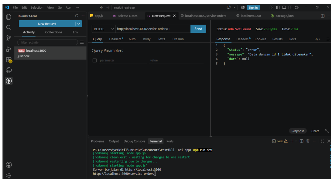
Gambar 10. Pengujian DELETE //service-orders/1.
